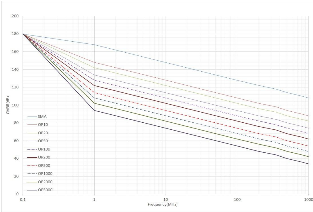
▲ Amplitude-frequency characteristics of different SigOFIT probes Attenuator
