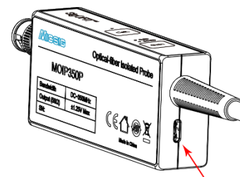
Power probe with standard Type-C charger
