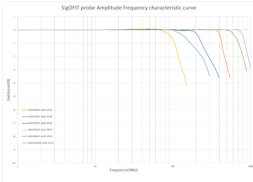
▲ Amplitude-frequency characteristics of different SigOFIT probes Attenuator
