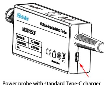
Power probe with standard Type-C charger
