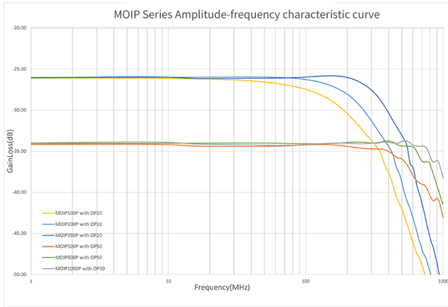
▲ Amplitude-frequency characteristics of different SigOFIT probes Attenuator
