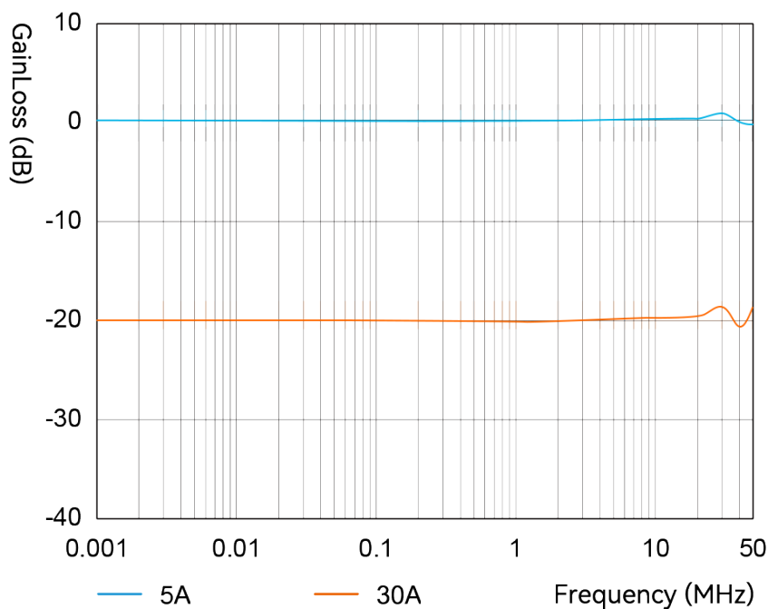
Figure 14: Amplitude-frequency characteristic curve CP503B
