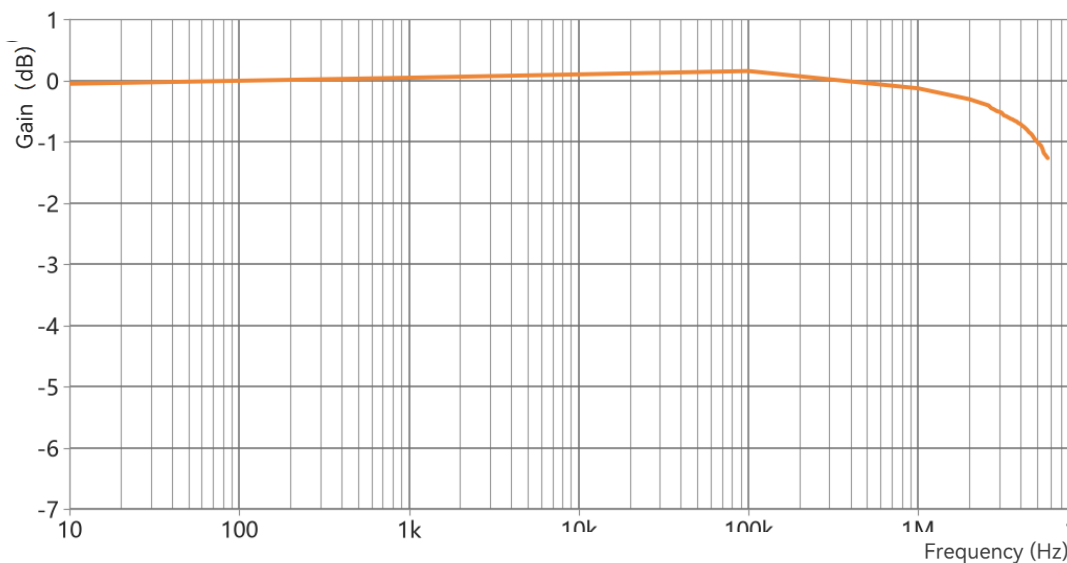
Figure 2: Amplitude-frequency characteristic curve CP5005
