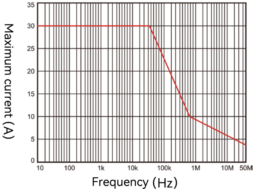
Figure 13. Maximum Current VS Frequency CP503B
