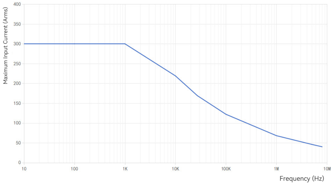
Figure 3. Maximum Current VS Frequency CP3008
