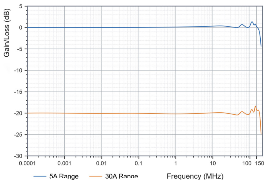
Figure 10: Amplitude-frequency characteristic curve CP1003B
