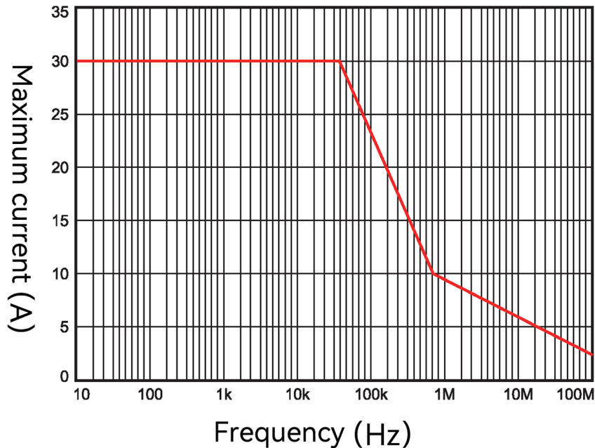
Figure 11: Maximum Current VS Frequency CP1003B
