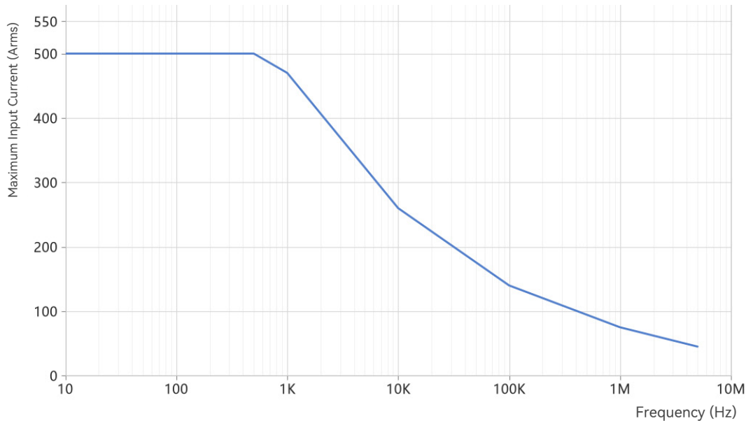
Figure 1. Maximum Current VS Frequency CP5005
