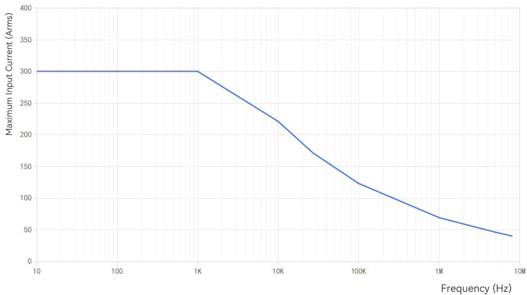
Figure 5: Maximum Current VS Frequency CP3005
