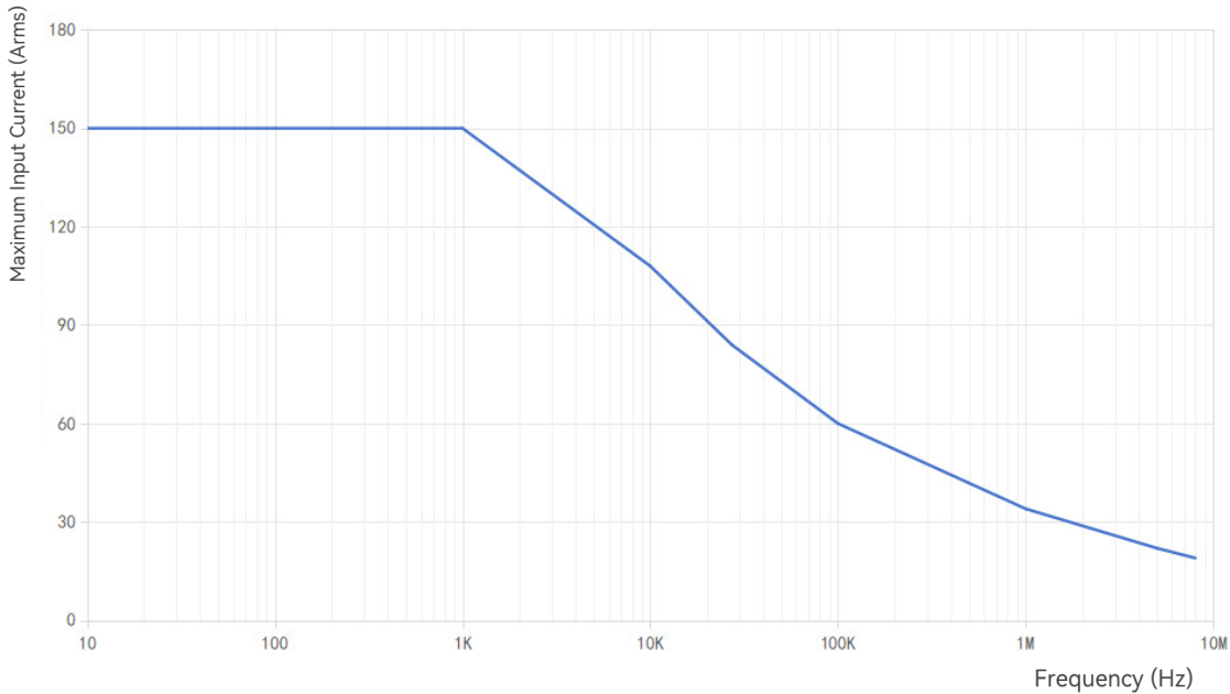
Figure 7. Maximum Current VS Frequency CP1510
