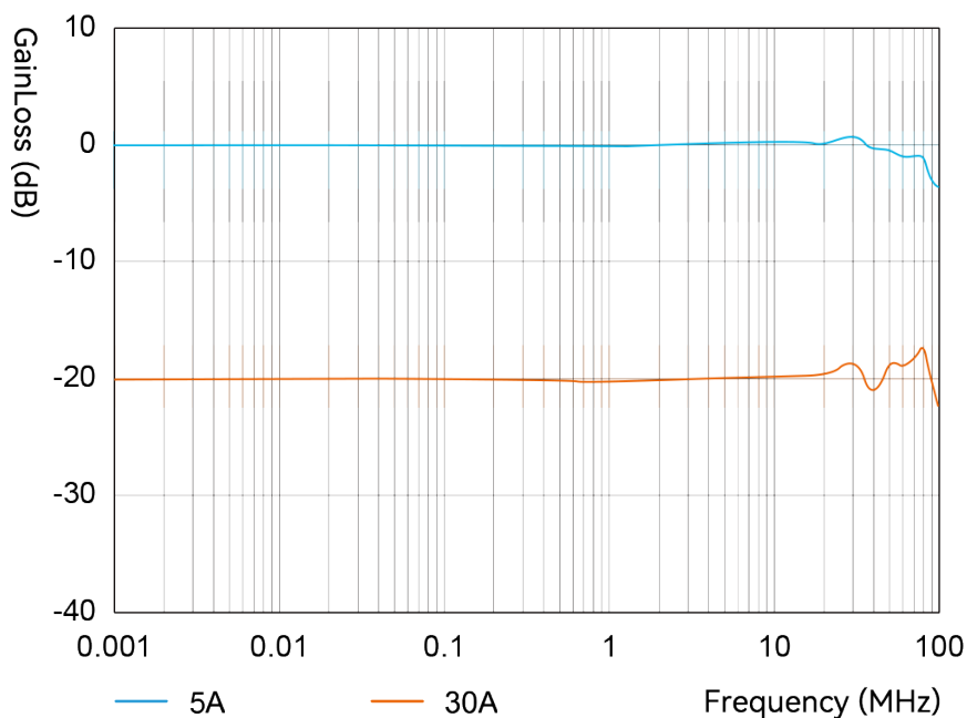
Figure 12: Amplitude-frequency characteristic curve CP1003B
